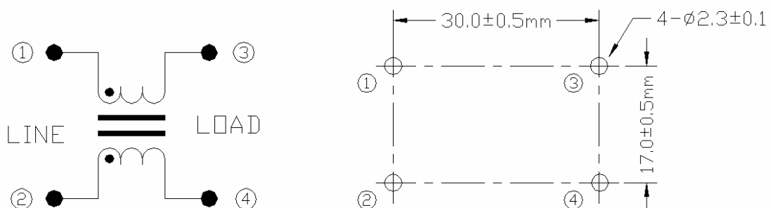
Minimum PCB piercing plan
